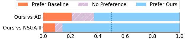
Figure 2. MOS listening test preference distribution.
