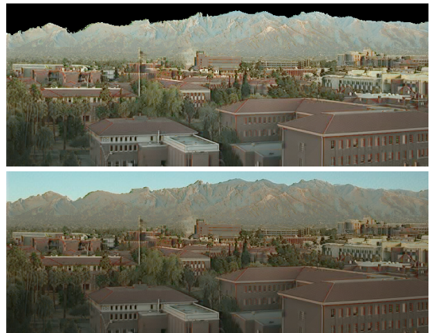
Figure 6: Top: Skylight image. Bottom: Reconstructed sky image.
